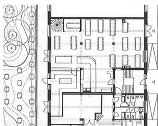
Grundriss Restaurant
